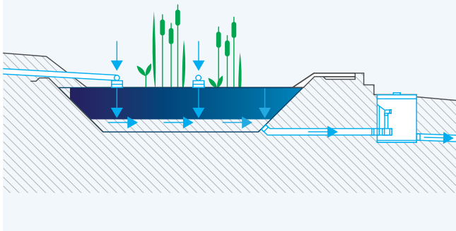
Type 1 - Vertical flow
