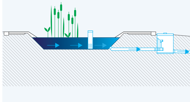
Type 2 - Horizontal flow
